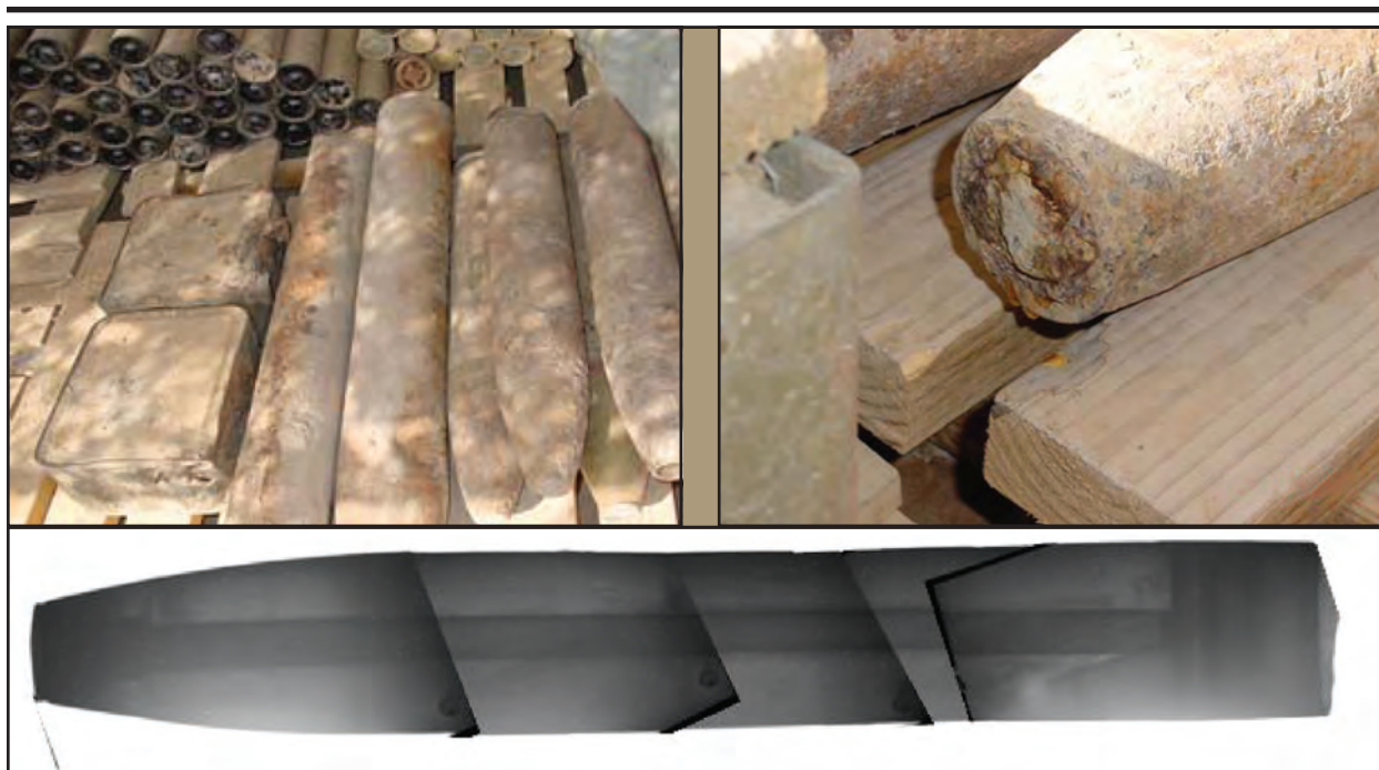
Figure 7. Photos and x-ray of SAKR-18 rockets.
